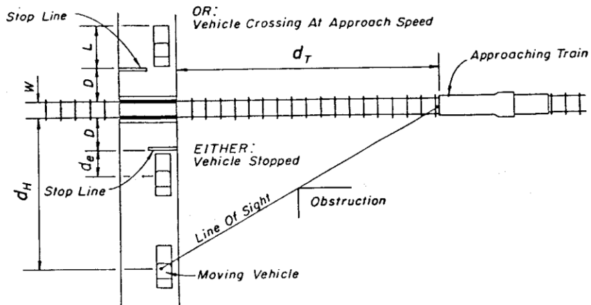
FIGURE 7 – 1 VISIBILITY TRIANGLE AT RAILROAD CROSSINGS
