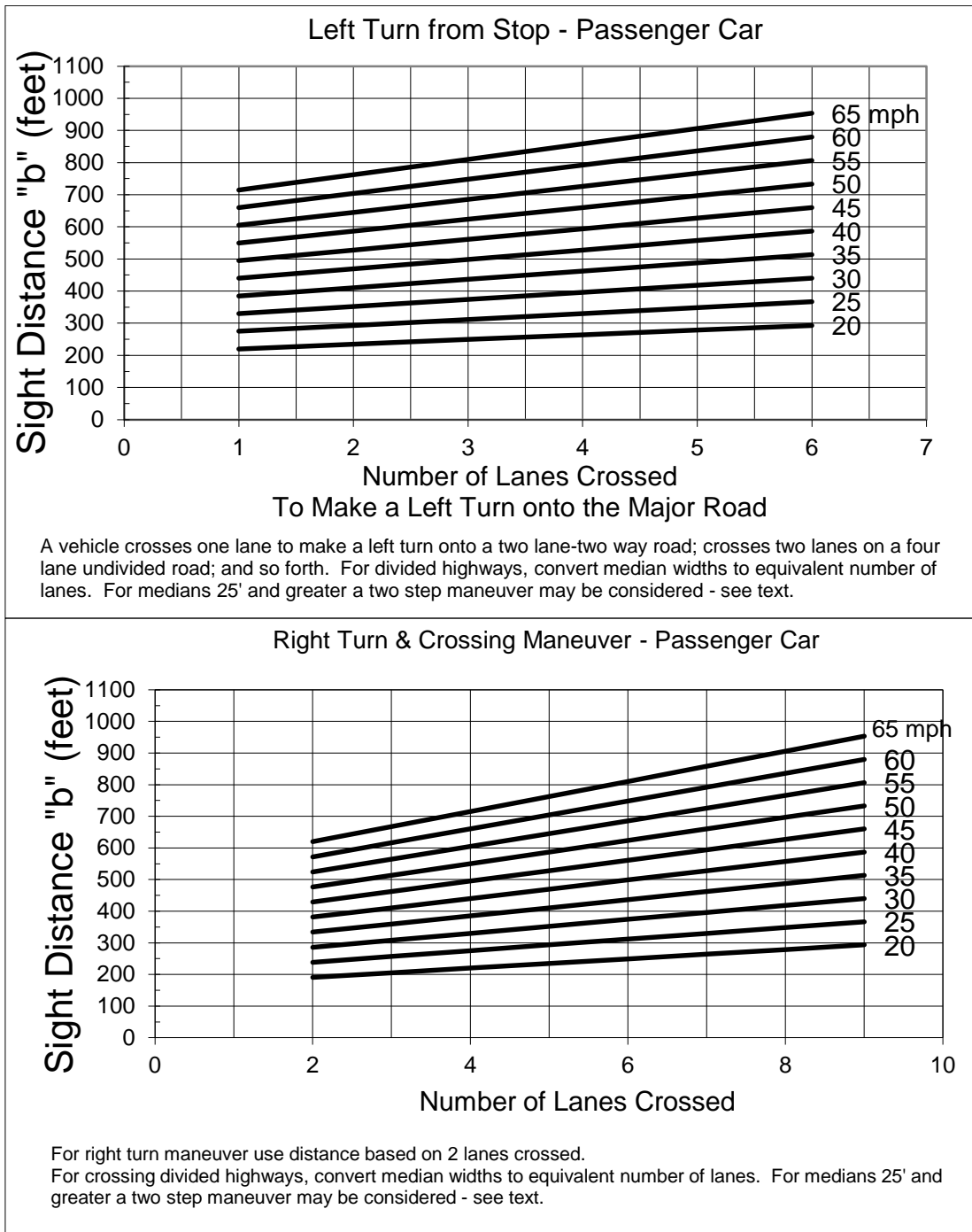
FIGURE 3 – 8 INTERSECTION SIGHT DISTANCE
